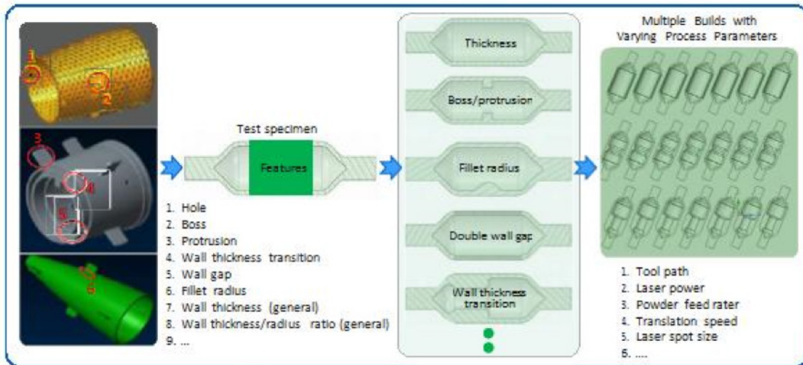
An example of a feature-based qualification test process where multiple samples are printed in a single build with varying process parameters to capture different additively built characteristics and feature geometries.
