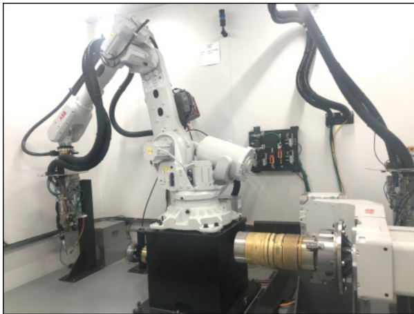
Wolf Robotics Laser Wire AM System that resides in the Manufacturing Demonstration Facility at Oak Ridge National Labs (left). Schematic showing the elements and interfaces of the framework being developed (right).
