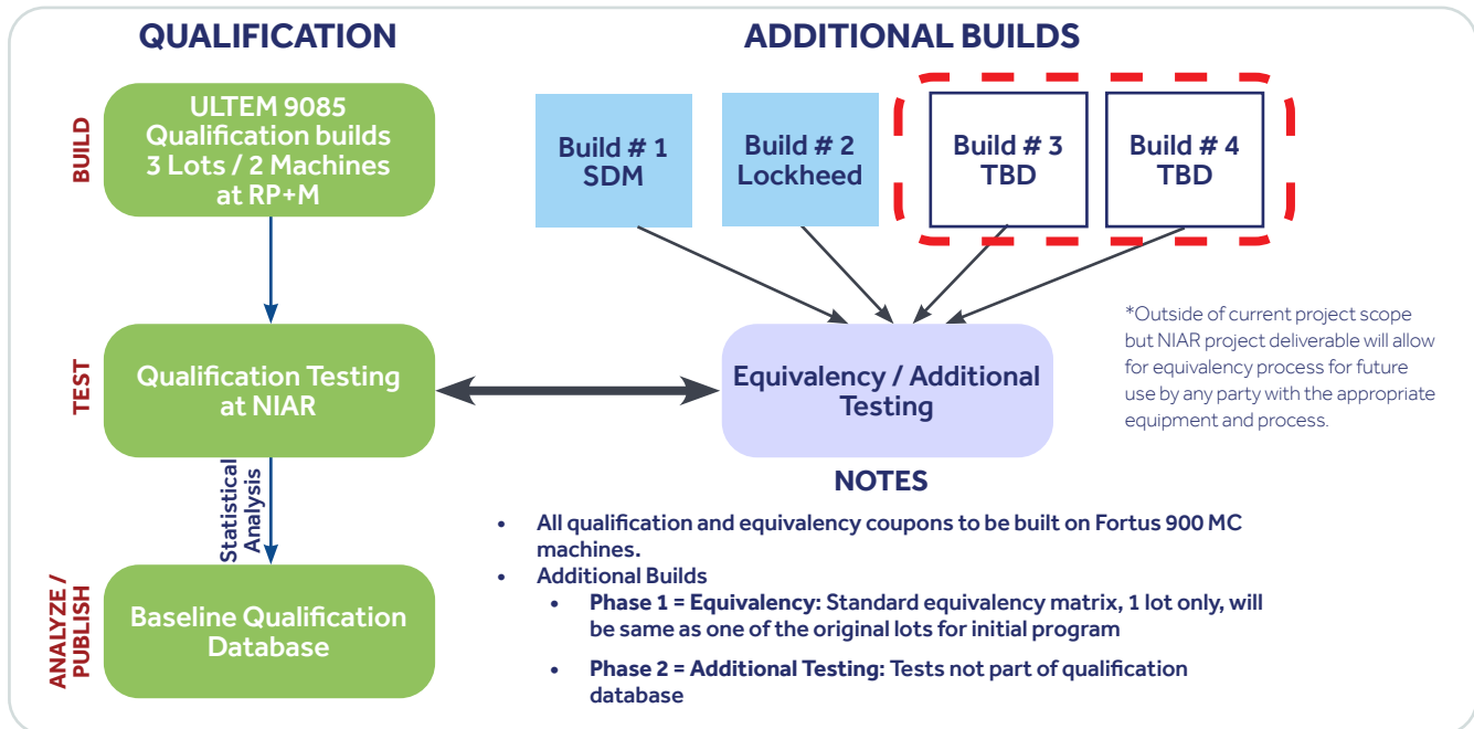
Overview of project plan for qualification and equivalency testing for FDM printing of ULTEM™ 9085.
